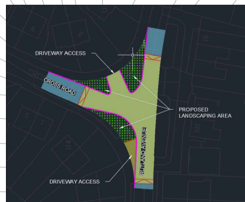
REMOVAL OF EXISTING SPEED HUMP AND EXISTING JUNCTION TO BE MODIFIED AS STANDARD T-JUNCTION WITH TABLE TOP WITH UNCONTROLLED PEDESTRIAN CROSSING FACILITIES
