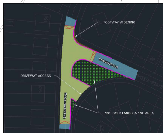
EXISTING JUNCTION TO BE MODIFIED AS STANDARD T-JUNCTION WITH TABLE TOP WITH UNCONTROLLED PEDESTRIAN CROSSING FACILITIES
